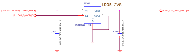
Rear-Slave AVDD 2.8V
