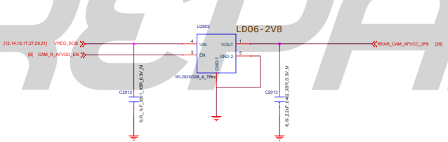
Rear-Main AFVCC 2.8V
