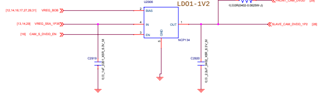
Rear-Slave DVDD 1.2V (Also 8M Front DVDD)
